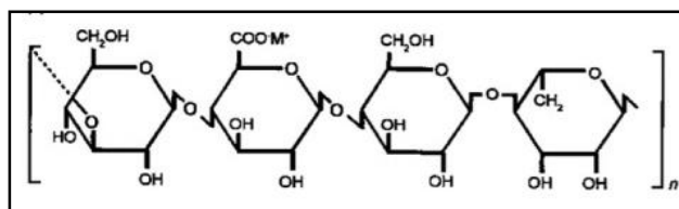
Fig. 1 Structure of Gellan Gum
