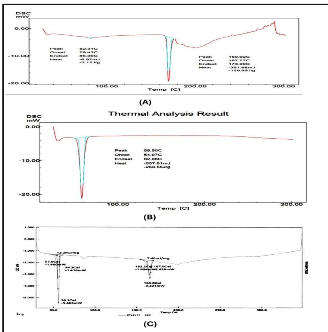
Figure 1: DSC of (A) Ketorolac tromethamine (B)poloxamer 407 (C) physical mixture Ketorolac tromethamine and poloxamer 407(1:1 w/w)
