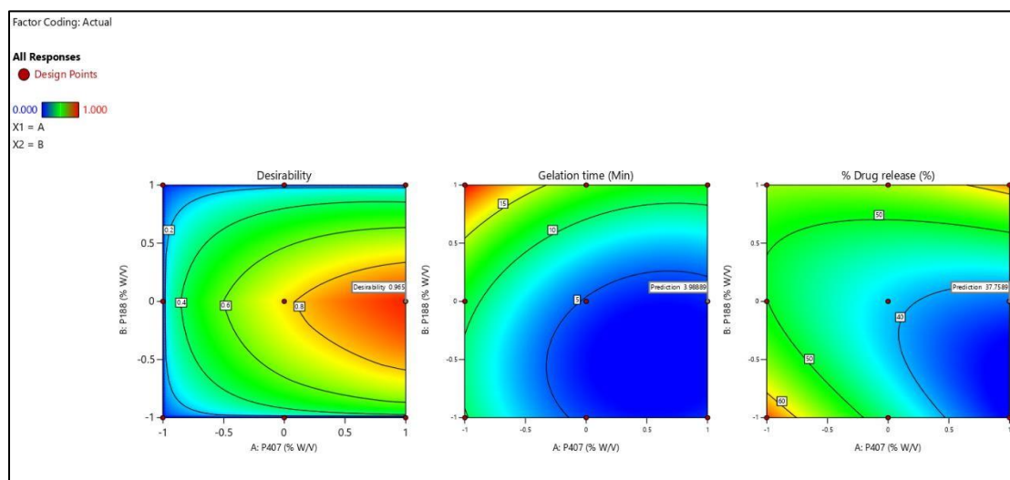
Figure 5: Optimization of desirability function by Design-Expert 13
