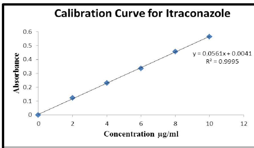
Figure 4: Standard calibration curve at 255 nm
