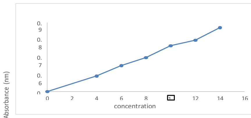
Figure 4: Standard calibration curve at 255 nm
